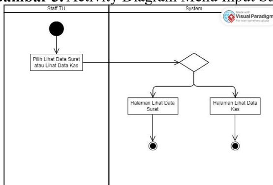
Gambar 4. Activity Diagram Menu Lihat Data Surat
