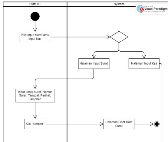
Gambar 3. Activity Diagram Menu Input Surat
