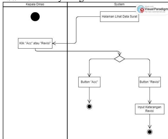
Gambar 5. Activity Diagram Menu Persetujuan Surat
