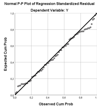
Grafik 1 Uji Normalitas Probability Plot
